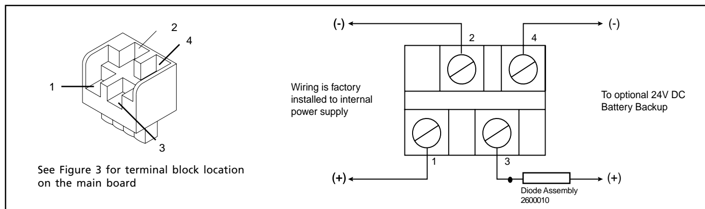
Figure 4. Wiring to Terminal Block TB1 Input Circuit
